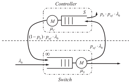
Fig. 4. A simple model of an OpenFlow switch.
