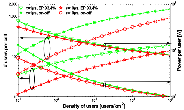
Fig. 6. Right y axis: Minimum amount of power consumed per user. Left y axis: Optimal number of users per cell as a function of user density. Base stations are distributed according to the Poisson layout.
