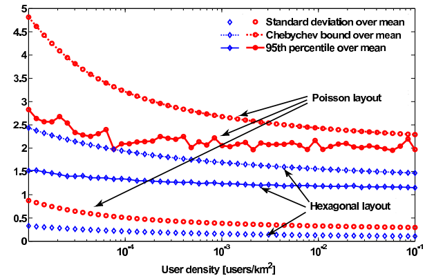
Fig. 7. Standard deviation, 95th Chebyshev bound and 95th percentile of the per-bit delay. All quantities are normalized over an average per-bit delay of 1 \mu s .
