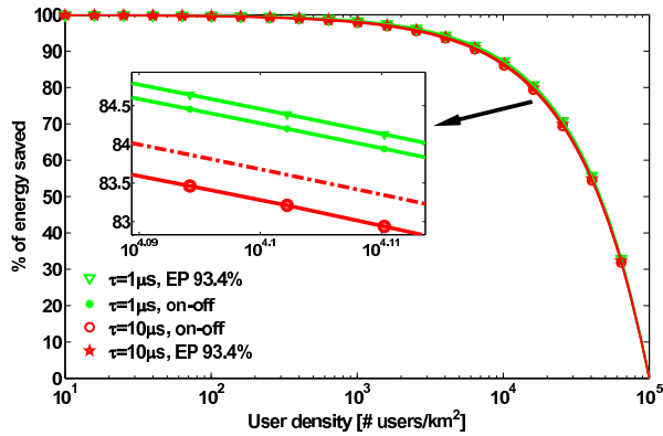
Fig. 4. Percentage of energy saved with sleep modes in a Poisson layout, with respect to the energy consumed at a peak user density of 10^5 users/km 2 .
