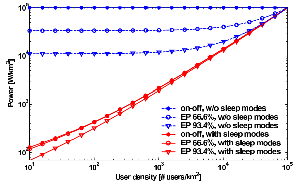
Fig. 5. Minimum power consumed by base stations per km 2 , as a function of user density. Base stations layout is Poisson, and \tau = 10 \mu s .
