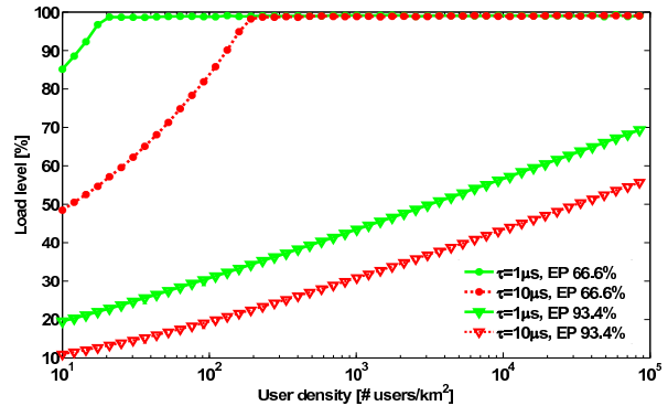
Fig. 3. Average utilization level of base stations at the optimal base stations density versus user density for a Poisson base stations layout.
